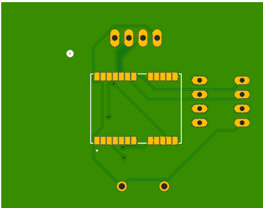
Figure 8.7. GPS Module PCB (Bottom Side)
