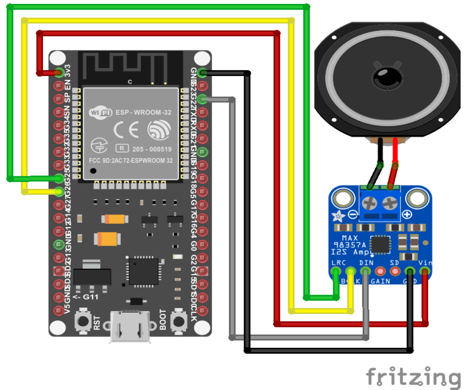
Figure 6.11. I2S ESP 32 Setup Example (Pending Permission).
