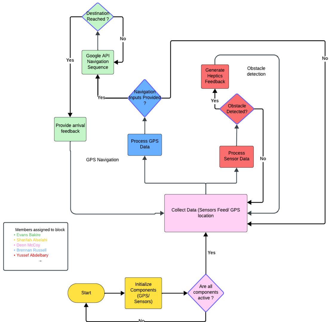
Figure 2.4. Software design flowchart.
