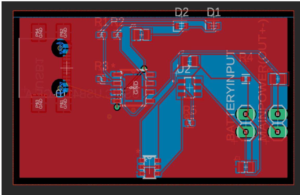
Figure 8.3. TP4056 Module PCB Layout.
