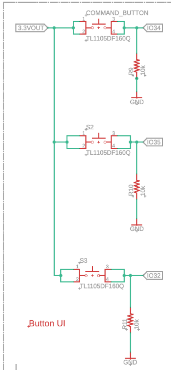
Figure 6.6. Buttons and resistors for UI commands Schematic.
